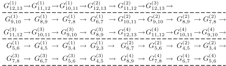
Figure 3.2: Regrouped sequence of Givens rotations.
