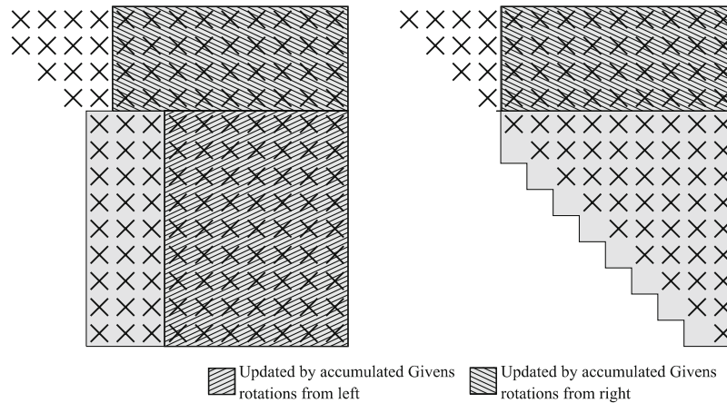
Figure 3.3: Illustration of panel-wise factorization for j_c = 3 , n_b = 3 .
