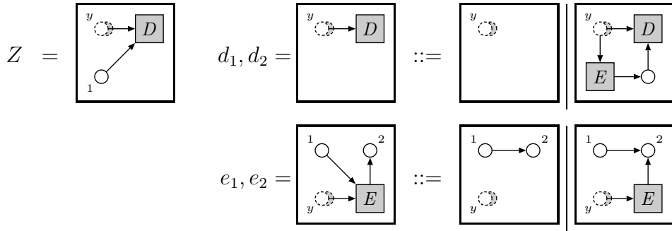
Figure 9: A star grammar deriving all directed acyclic graphs
