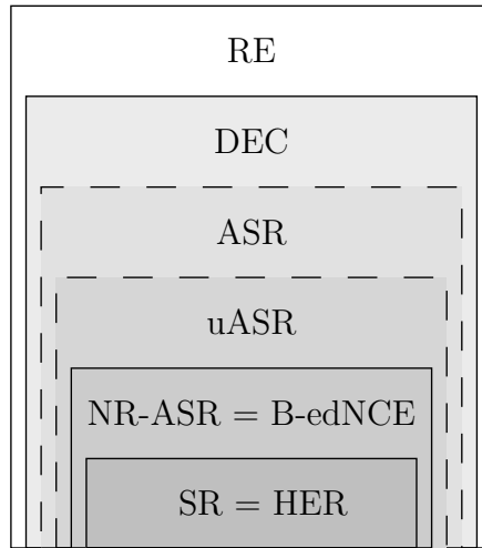
Figure 12: Relation of languages generated by star replacement
