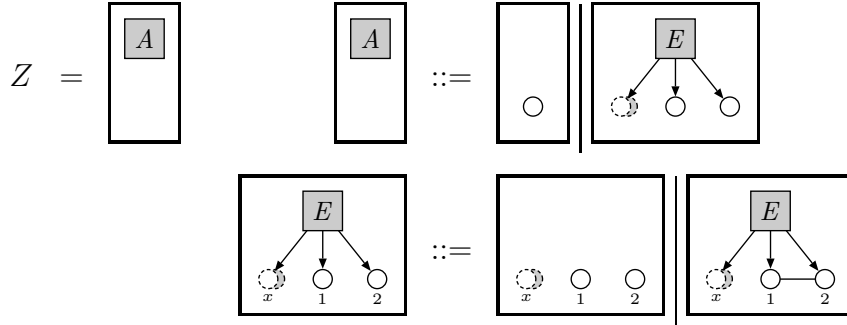
Figure 11: A uniform star grammar deriving all graphs
