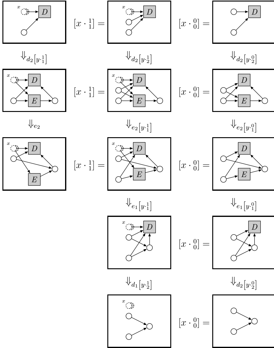
Figure 10: Derivations of a directed acyclic graphs
