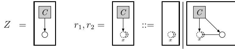
Figure 6: Adaptive star grammar for deriving complete graphs
