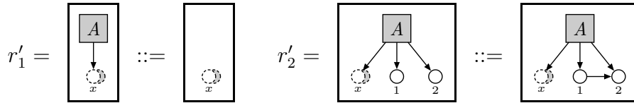
Figure 7: A star grammar deriving all graphs
