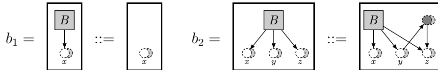
Figure 8: A star grammar deriving all bipartite graphs
